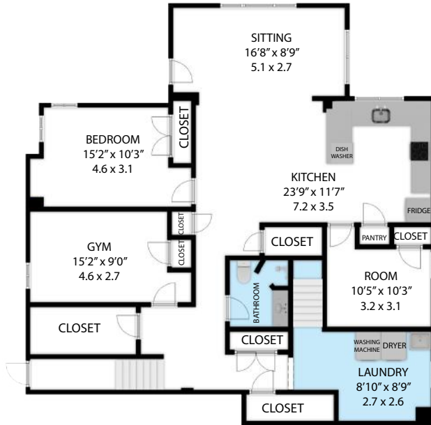
LOWER LEVEL 1,395 SQFT - 130 SQ.M
