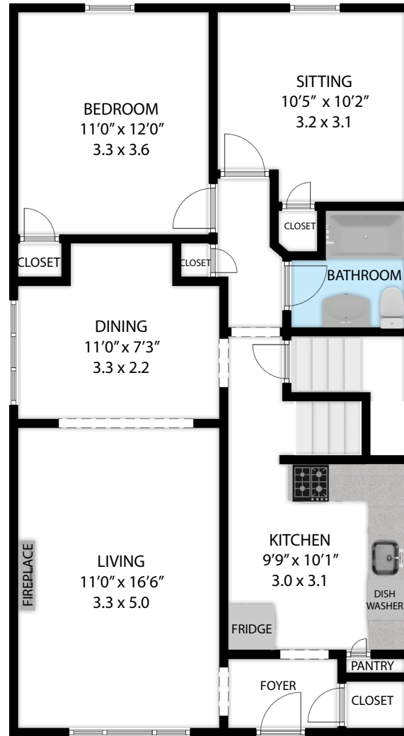
MAIN LEVEL 893 SQ.FT - 83 SQ.M
